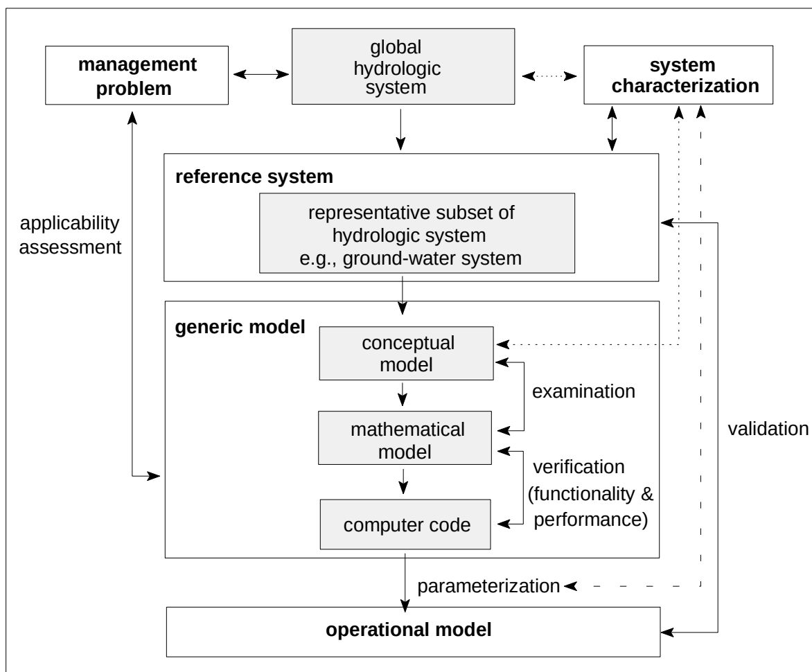
Figure 1-1. Code development and testing concepts.
